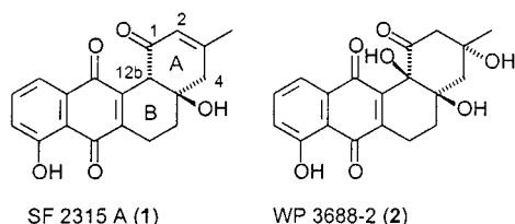
Scheme 1. Examples of angucyclines of the SF 2315 and SS 288Y types
